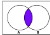
A \cap B
