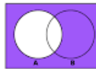
A' is the complement of A
