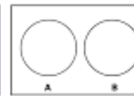
A and B are Disjoint sets
